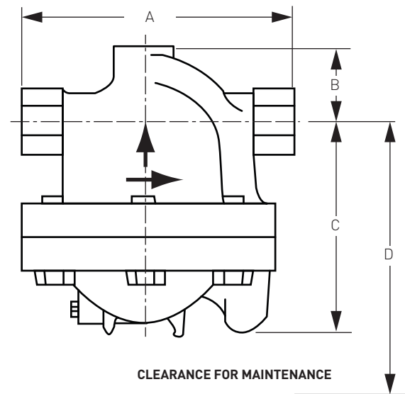
FXT700 Series Variable Orifice Steam Trap Dimensions
