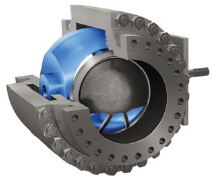
Figure 5.16 Ball-Style Valve with Attenuator to Reduce Hydrodynamic Noise
