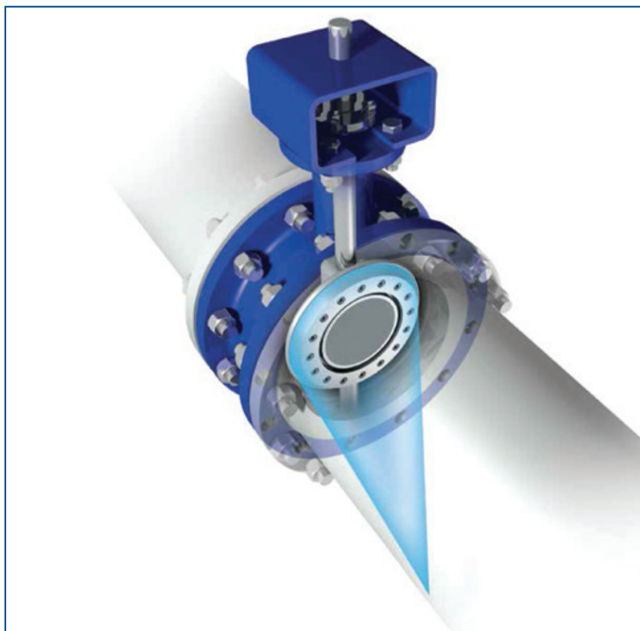
Cone-to-cone sealing principle in a triple offset valve (rotational movement)
