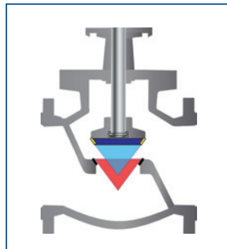
Cone-to-cone sealing principle in a globe valve (axial movement)
